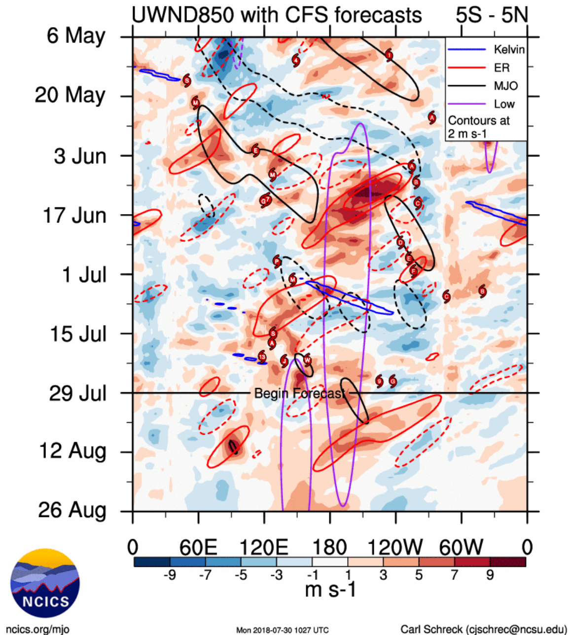
Figure 8: Anomalous 850-mb winds averaged near the equator. Over the past few days, trade winds have weakened in the central Pacific and are forecast to remain weak for the next several weeks by the Climate Forecast System. Figure courtesy of Carl Schreck.
