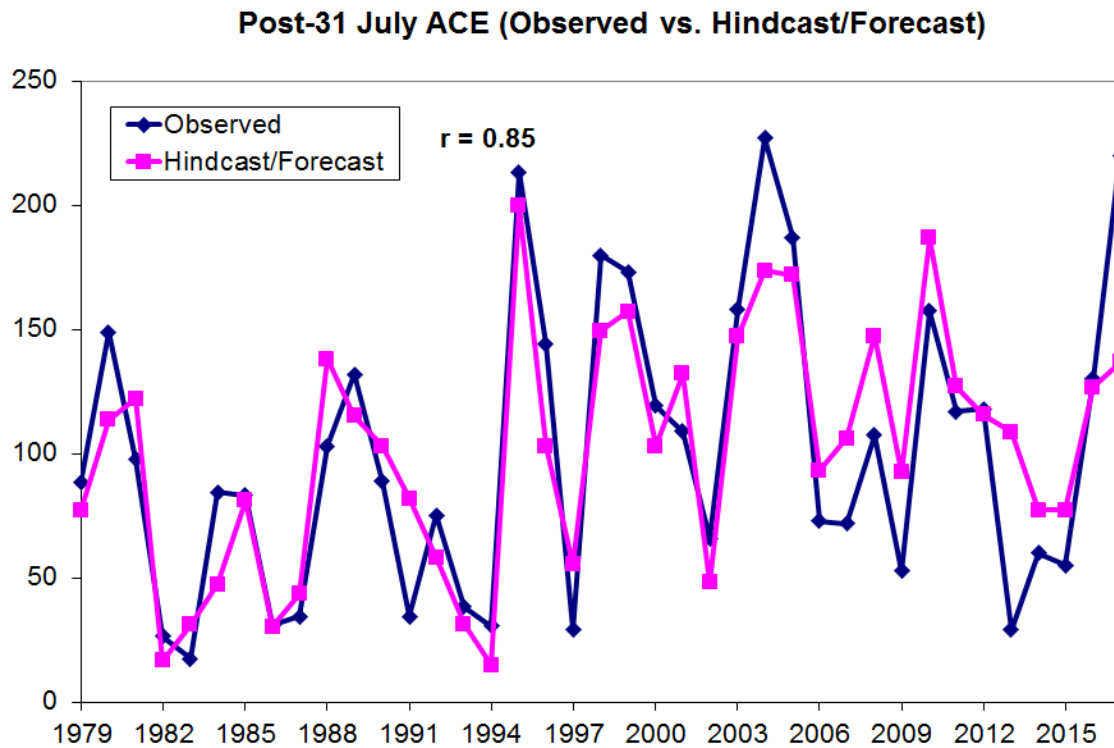
Figure 3: Observed versus hindcast values of post-31 July ACE for 1979-2017 using our current statistical scheme.
