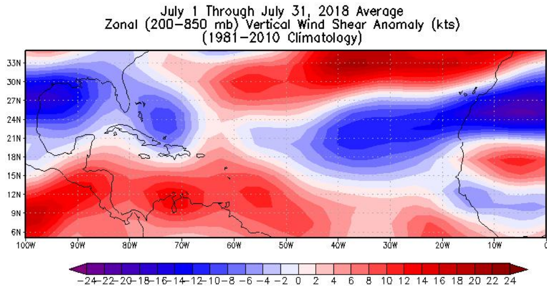
Figure 14: July 2018 averaged 200-850-mb zonal wind anomalies across the tropical Atlantic
